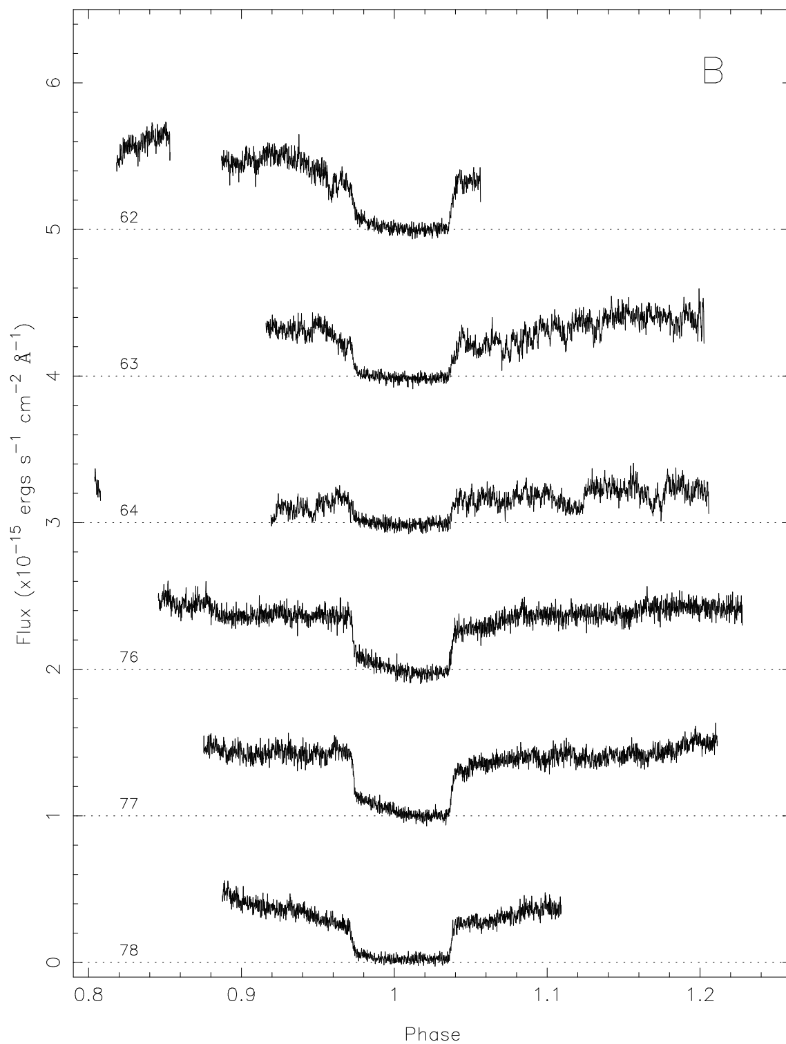
Figure 4.4: B -band light curve for all six cycles binned into 1 s time intervals and phased with respect to the ephemeris of Schwobe and Mengel (1997).
