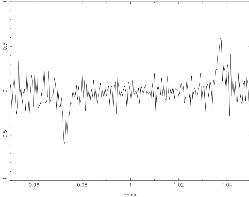
Figure 4.7: The mean of the six 3 s differential white light curves.
