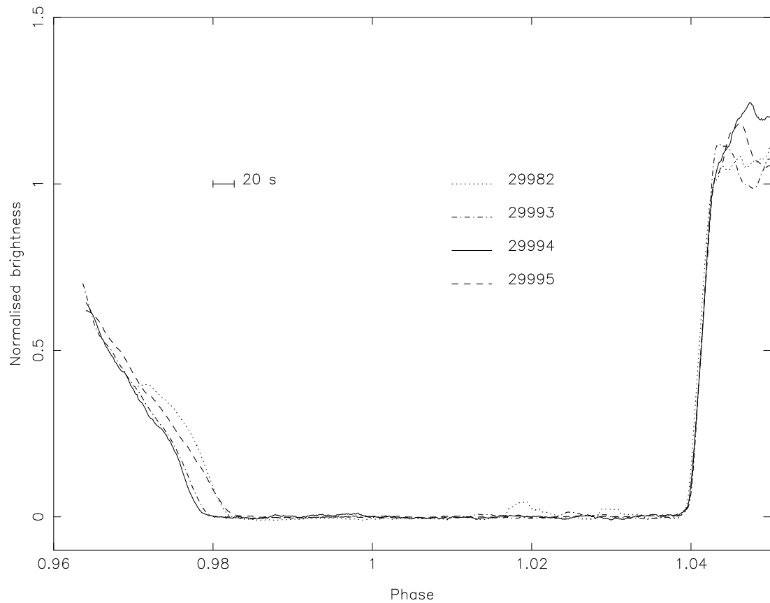
Figure 3.8: The ingress and egress of eclipses 29982 (dotted), 29993 (dash-dot), 29994 (solid) and 29995 (dashed) smoothed over a running average of 20s. The ordinates are normalised to 1 at the end of spot egress, and to 0 at total eclipse.
