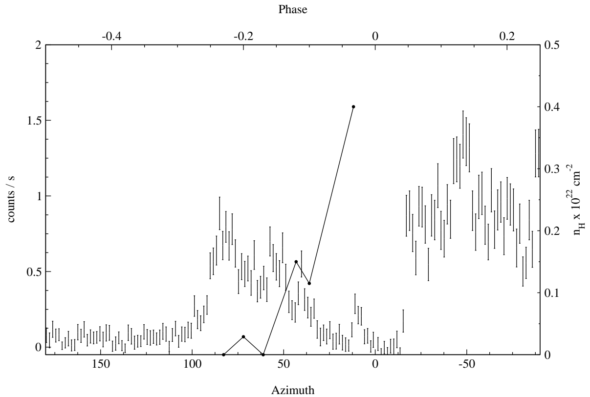
Figure 6.6: A plot of the absorption column density n_H versus azimuth plotted over the soft-band light curve. The absorption uses the lower abscissa and right-hand ordinate, while the soft-band light curves uses the upper abscissa and left-hand ordinate.
