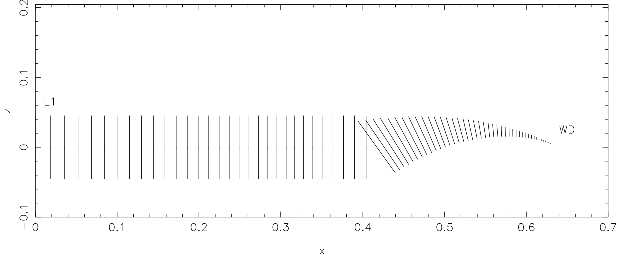
Figure 7.1: The accretion stream cross-section structure for the irradiative model.
