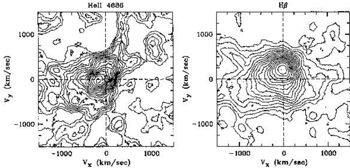
Figure 7.12: The Doppler tomograms of EP Dra from Schwobe and Mengel (1997).
