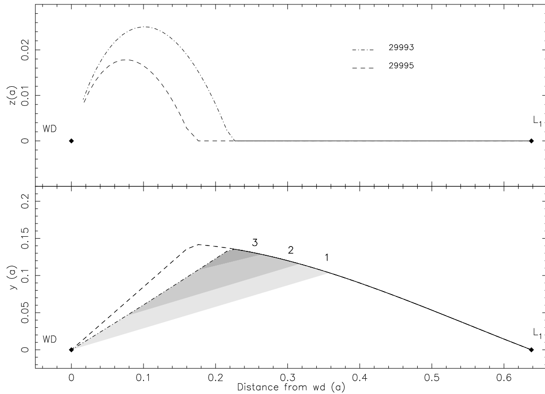
Figure 3.13: The upper plot shows the model stream points for cycles 29993 and 29995 looking parallel to the orbital plane, while the lower plot shows them looking down onto the orbital plane. The difference in the stream trajectories is evident. The shaded regions are three equal phase intervals encompassed by the ingress of the white dwarf and the final ingress of the threading region for cycle 29993. These correspond to those parts of the stream used to form sections 1, 2 and 3 in Figure 3.14. (For cycle 29995 the definitions are equivalent.)
