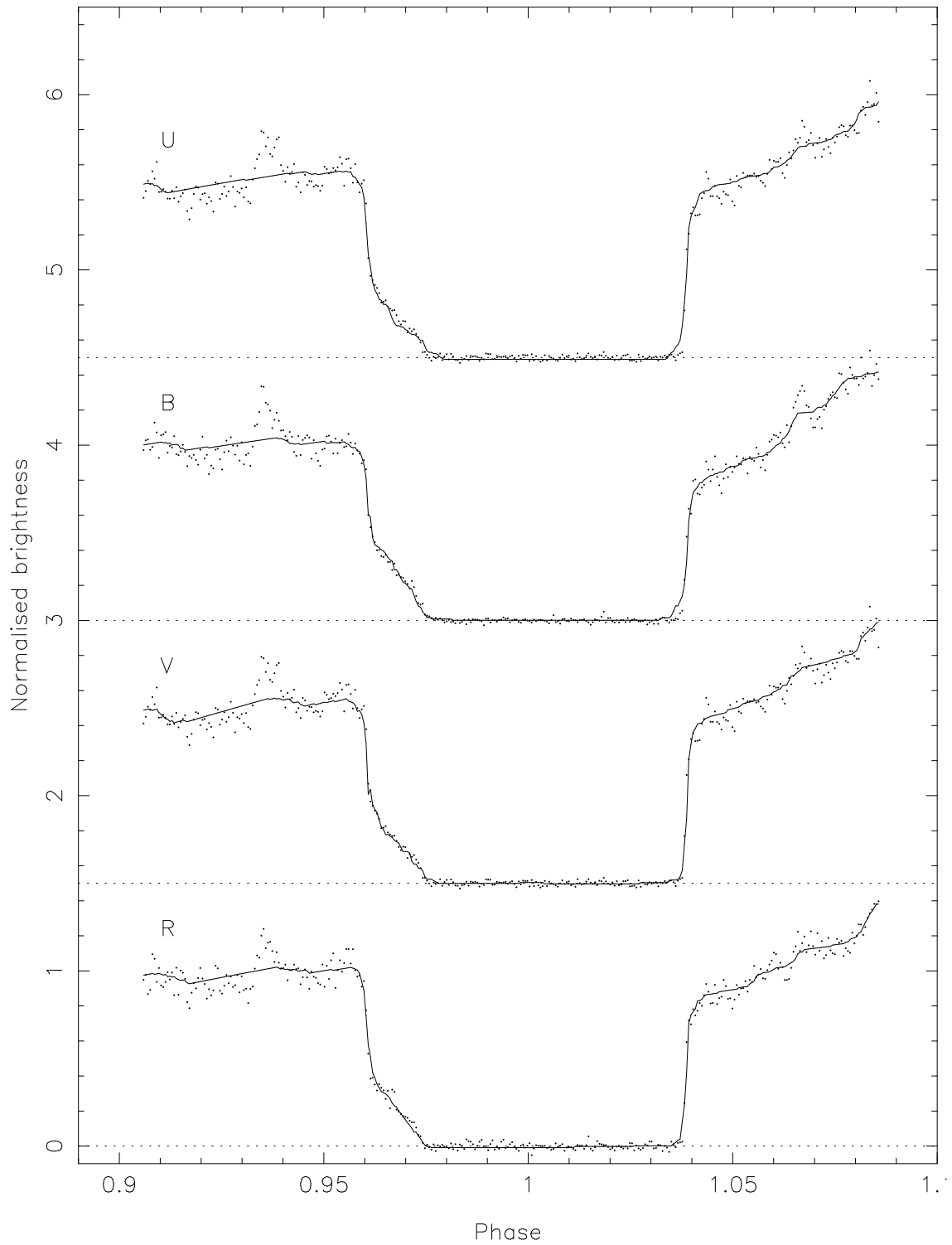
Figure 5.4: The model fits (solid line) to the observed UBVR_c -band light curves (dots) of HU Aqr. Each light curve and fit is offset vertically by 1.5 for clarity.
