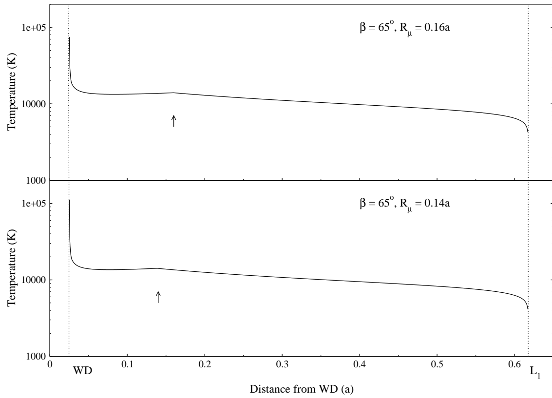
Figure 7.7: As for Figure 7.6, but for \beta = 65^\circ and R_\mu = 0.16a and 0.14a .
