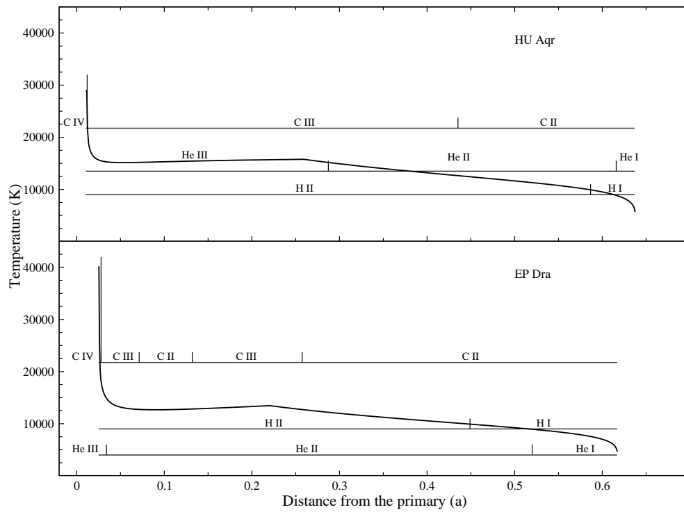
Figure 7.10: The location of the dominant ionized species along the accretion stream for H, He and C from the temperature profiles of HU Aqr 29993 and EP Dra ( R_{\mu} = 0.22a ). The short vertical lines divide the stream into region where the indicated species dominates (Kallman and McCray, 1982, see Figures 7.8 and 7.9).
