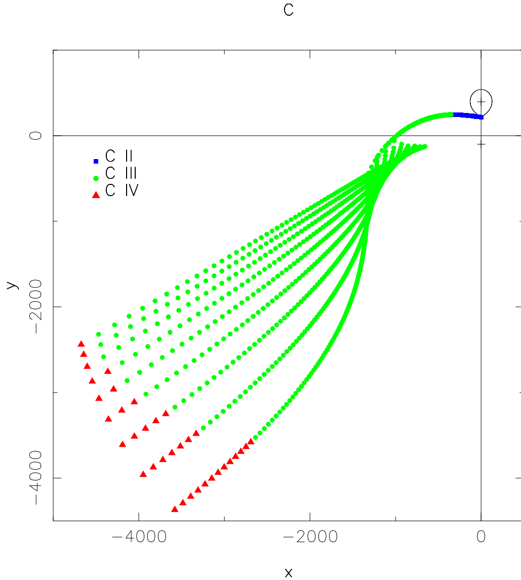
Figure 7.15: As for Figure 7.14, but for C ions. Note from Figure 7.8 that the C_{\text{v}} always dominates over C_{\text{iv}} , but is excluded from the figure for clarity. C_{\text{iv}} is included as this is observed in Doppler maps of polars.
