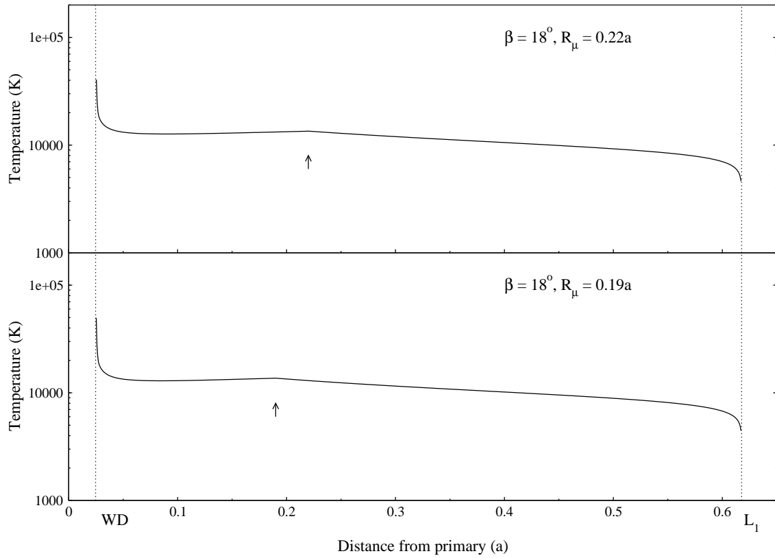
Figure 7.6: The temperature structure of the model stream is shown as a function of distance from the primary (in units of the binary separation), for EP Dra with \beta = 18^\circ . The upper plot represents R_\mu = 0.22a and the lower R_\mu = 0.19a . The position of L_1 and the surface of the primary are indicated with a dashed line and R_\mu with a short arrow.
