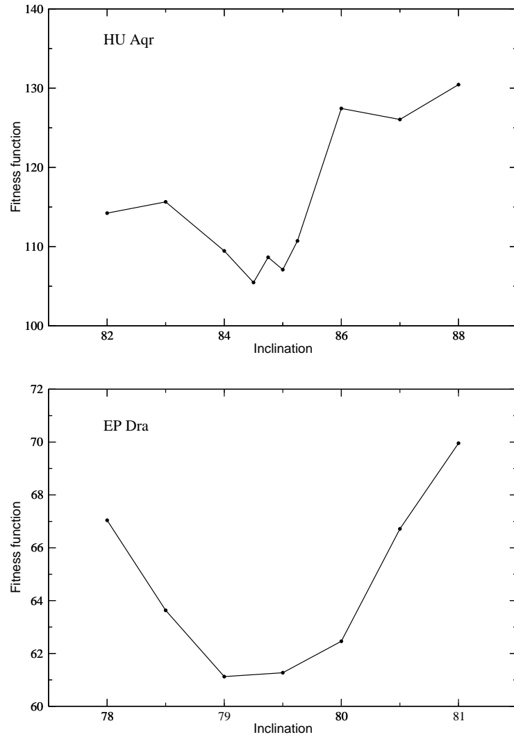
Figure 5.2: The upper plot shows the fitness function for a range of values of inclination for the V -band of cycle 29995 of HU Aqr, and the bottom plot that for cycle 56976 of EP Dra.
