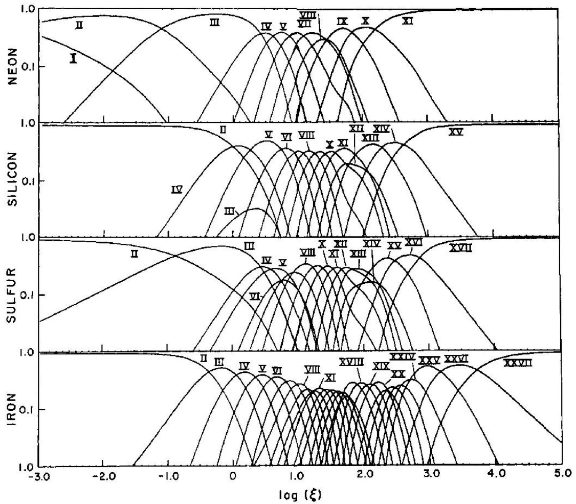
Figure 7.9: As for Figure 7.8. From Kallman and McCray (1982).
