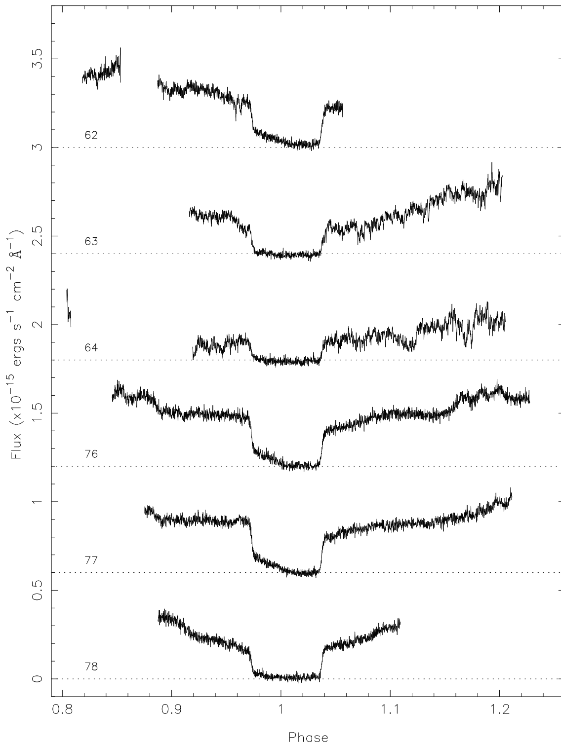
Figure 4.1: White light curves for EP Dra in 1 s time bins. Each cycle is offset vertically by 0.6 \times 10^{-15} \text{ ergs s}^{-1} \text{ cm}^{-2} \text{ \AA}^{-1} , and phased according to the ephemeris of Schwobe and Mengel (1997).
