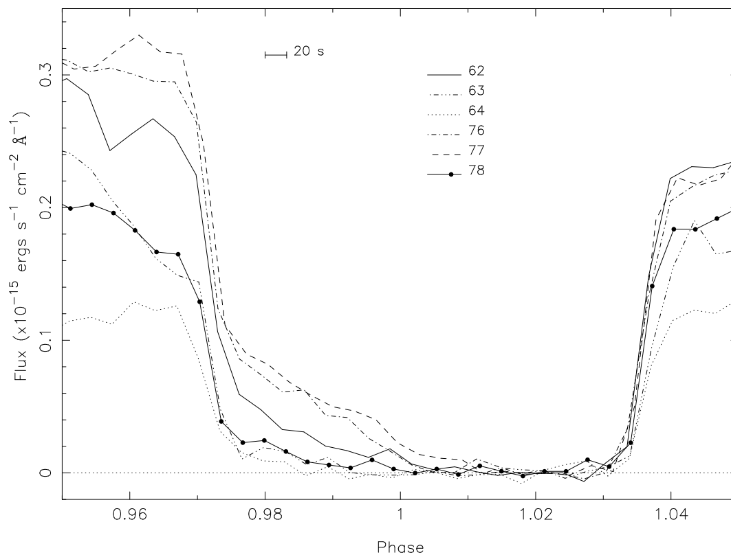
Figure 4.9: The six white light curves centred on the eclipse by the secondary. They have been binned into 20s time bins, which removes any features related to the eclipse of the white dwarf and the accretion region. The contribution from the secondary has been subtracted.
