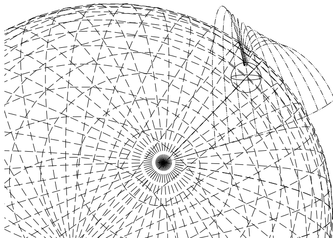
Figure 4.10: Plot of the geometry of EP Dra consistent with a variable brightness stream for \phi = 0.98 . The magnetic field lines are still visible, causing a long stream ingress in the light curves for bright stream material confined to these field lines. The magnetic pole is located at \beta = 18^\circ and \zeta = -17.0^\circ (assuming the values for the accretion region in Remillard et al. (1991) are the same as the magnetic pole).
