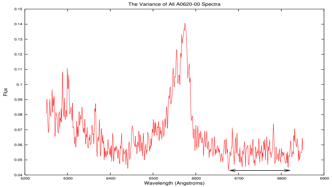
Figure 3.4: The associated standard deviation of the mean normalised spectrum in Figure 3.3 shown on a larger scale. The region defined by the arrow indicates the least varying region of the spectrum. The mean flux of this region is the constant used for normalisation.
