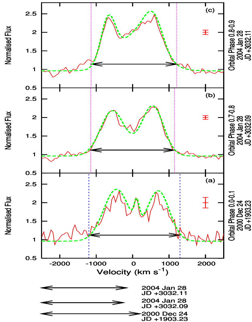
Figure 4.18: A comparison of the line widths of \text{H}\alpha . The individual spectrum (line) in each panel is plotted with its error and the fit using a 3 Gaussians function (dashes). The two vertical lines in each panel indicates the width of the \text{H}\alpha line, marked out by the horizontal double arrowed line at 10% of the lower peak. The lowest panel (a) shows the spectrum with the widest line width, taken on 2000 Dec 24 (JD +1903.23). The spectrum in panel (b) shows the spectrum with the narrowest line width, taken on JD 3032.09 (2004 Jan 28). The spectrum in panel (c) is taken on the same observing night JD 3032.11 (2004 Jan 28), however the line width is significant larger than the other spectra taken in the same observing run. The length of the arrows corresponding to the width of the spectra are compared below the plots.
