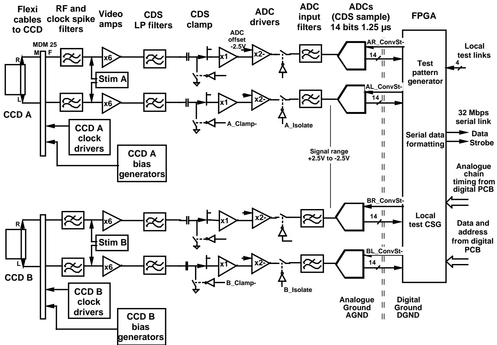
MSSL/SLB-EIS/DD/022.01 ROE Analogue PCB Block Diagram
