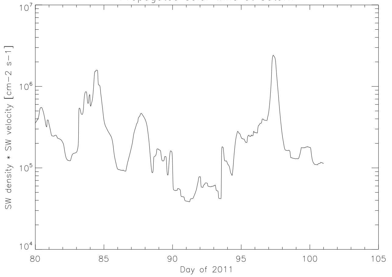
Propagated solar wind at Saturn
