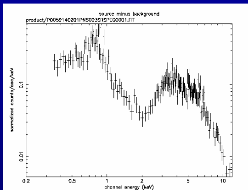
X-ray spectrum
