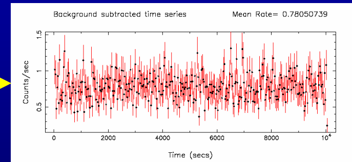
time series
