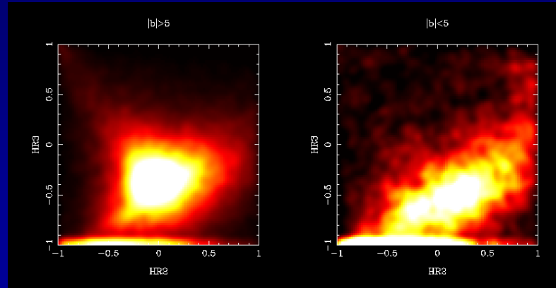
X-ray colour-colour plots
