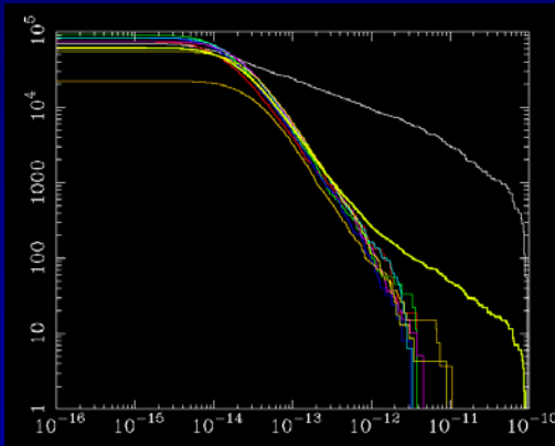
"raw" log N – log S
