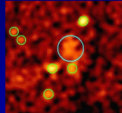
extended source detection & param
