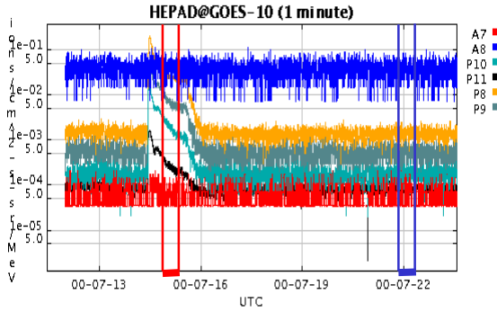
Fig. 2. GOES/HEPAD measurements of solar protons and \text{He}^+ . The 14 th and 21 st July flights are indicated by the red and the blue intervals respectively.
