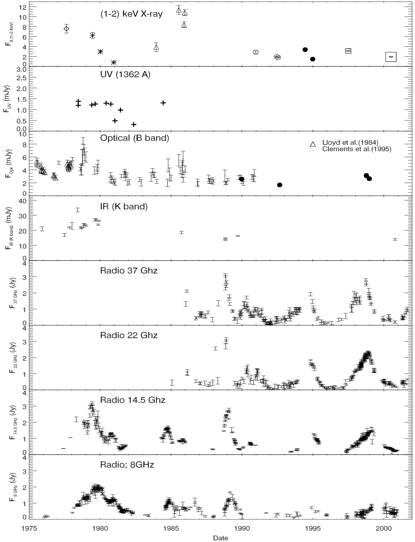
Figure 3.7: Multi-wavelength light curves of III Zw2 showing flux variations, with increasing wavelengths from top to bottom. (See §3 for the sources of data.)
