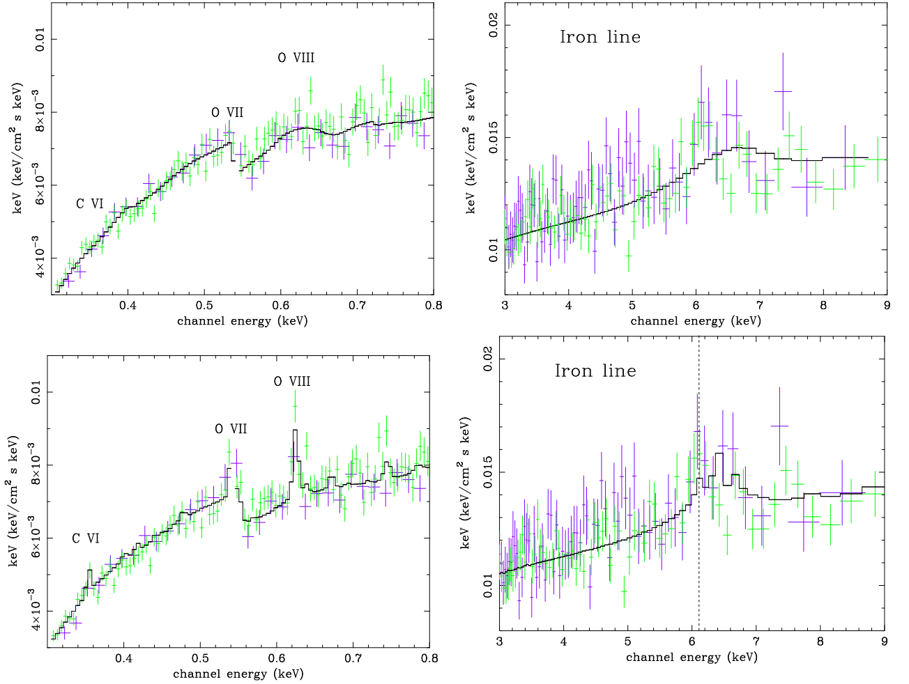
Figure 4.6: The hydrostatic balance reflection model (flare geometry) fit to the XMM-Newton data (MOS and PN data are represented by the dark and light points respectively. Although the RGS data were included in the model fits they are noisy and have been excluded from the plots for visual clarity). The top panels show the relativistically smeared spectrum and the bottom panels show the unsmeared spectrum in the observers frame ( z = 0.04732 ). The model reproduces the emission lump at low X-ray energies with a O VIII line. The model also produces O VII and C VI lines which become indistinguishable from the continuum when the spectrum is relativistically smeared. Most of the iron emission from the disk is at energies > 6.4 keV suggesting the presence of an ionised accretion disk in MCG-2-58-22. The position of the 6.4 keV line in the rest frame of the source is marked by a dashed line.
