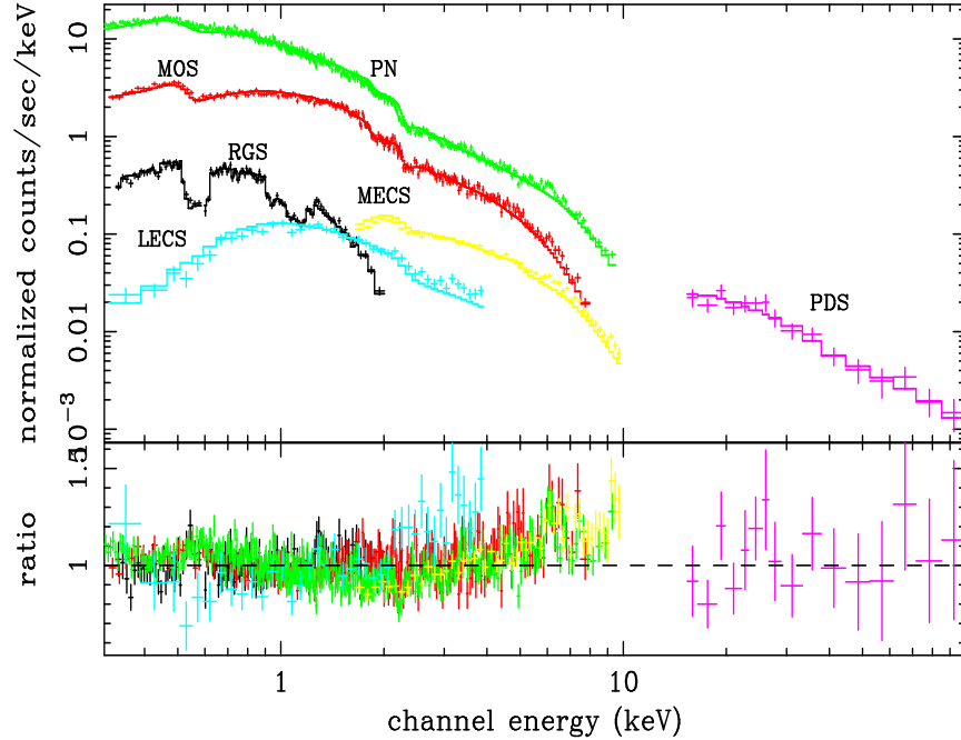
Figure 4.4: The 0.3–100 keV XMM – Newton and BeppoSAX spectra of MCG-2-58-22 (in the observers frame, z = 0.04732 ). The plot shows a power-law model fit to the data and the resultant fit residuals ( \Gamma = 1.86 \pm 0.01 , \chi^2/dof = 2311/1713 ). The Galactic column is fixed at N_H = 3.6 \times 10^{20} \text{ cm}^{-2} .
