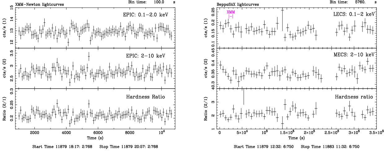
Figure 4.1: Left :Light curves and hardness ratio for the 10 ks XMM – Newton exposure Right : Light curves and hardness ratio for the long BeppoSAX exposure. The time of the XMM – Newton observation is marked by the small bracket in the upper right panel.
