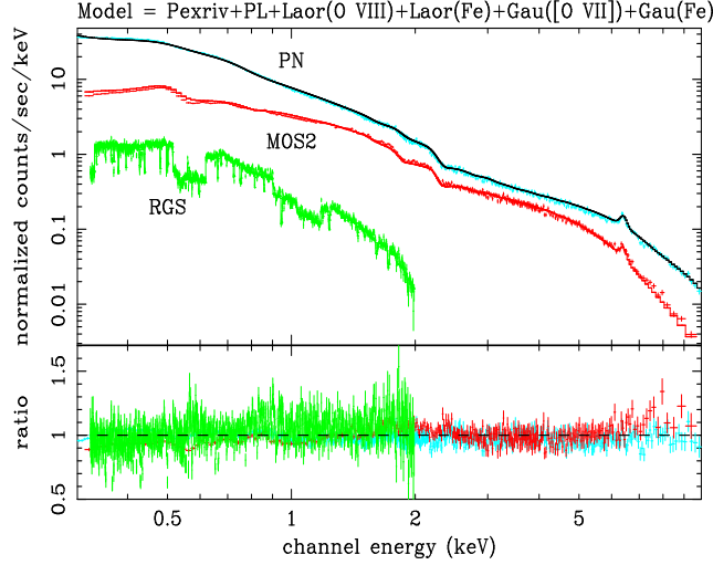
Figure 5.5: The PEXRIV(PL plus ionised reflection) + PL + 2Laor (O VIII, Fe) + 2gau (O VII, Fe) model fit to the integrated RGS and EPIC spectra. The neutral column density is fixed to the Galactic value of N_H = 1.32 \times 10^{20} \text{ cm}^{-2} . Although the fit residuals are reasonably distributed about the mean the fit statistics are unacceptable ( \chi^2/\text{dof} = 6757/2438 ). See Table.5.2 for details.
