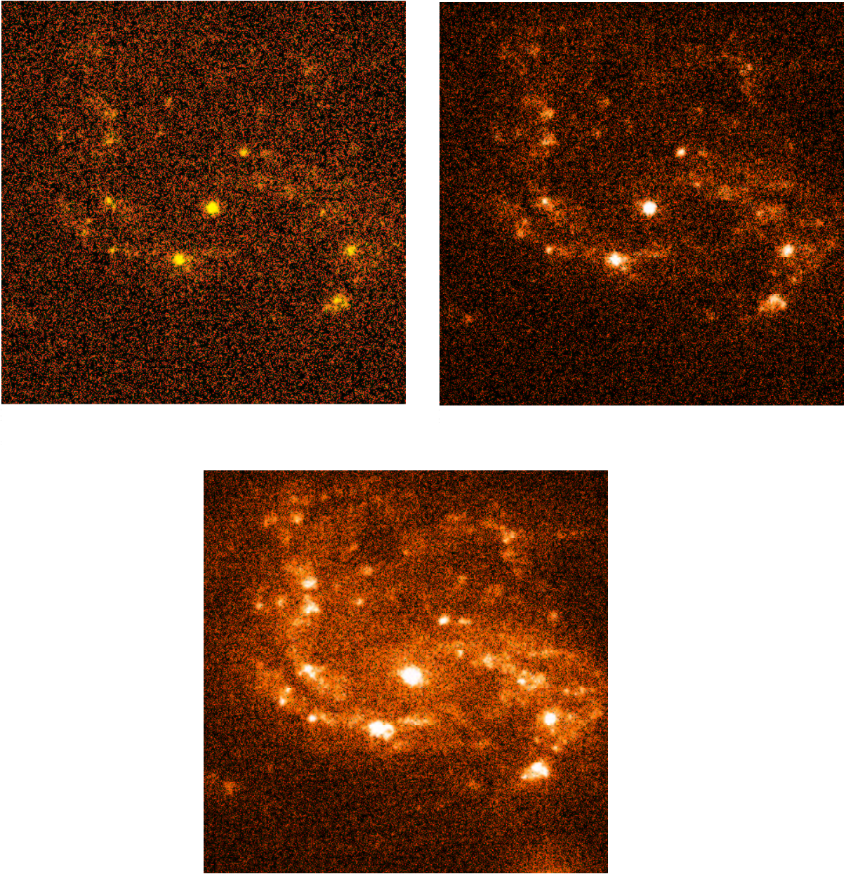
Figure 5.1: OM images of the NGC 4051 galaxy taken with the UVW2 (1800–2600 Å , top left ), UVM2 (2000–2800 Å , top right ) and UVW1 (2400–3600 Å , bottom ) filters. The central source and the spiral arms of the galaxy are clearly visible in all three filters. The nuclear source is brighter in the UV than the spiral arms
