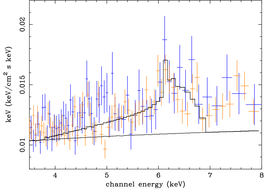
Figure 4.5: The plot shows the best fit model to the iron line profile (in the observers frame, z = 0.04732 ). The model includes a power-law, an ionised relativistic Fe K_{\alpha} line ( E = 6.83 \pm 0.26 emissivity q = -2.99 \pm 0.67 and inclination i = 28^{\circ} \pm 10 ) and a narrow Gaussian at 6.4 keV. The plot shows data from the MOS (dark points) and PN (light points). The dark solid line is the power-law model and the dark stepped curve on top of it is a model comprising a Laor emission line, a narrow Gaussian and power-law.
