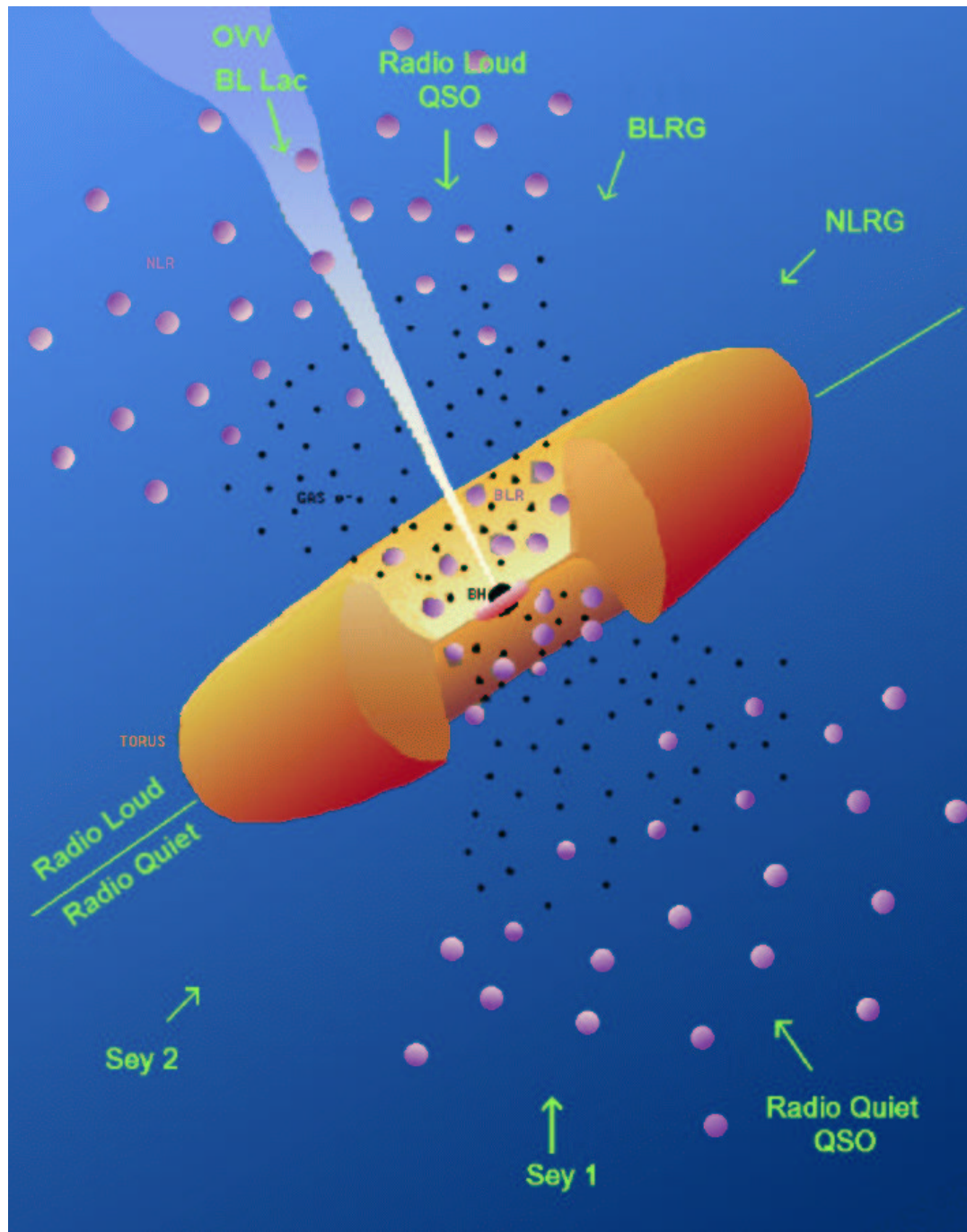
Figure 1.2: A schematic diagram of the physical structure of AGN ( credit : M. Urry & P. Padovani (Space Telescope Science Institute) isdc.unige.ch/Outreach/Help/help.html ). At the center lies the super-massive black hole surrounded by an accretion disk which fuels it and the relativistic jets. Further outward from the accretion disk are the dense rapidly moving broad line clouds (dark blobs). The central regions are surrounded by an optically thick dusty molecular torus. Beyond the torus are the low density slower moving narrow line clouds (light blobs)
