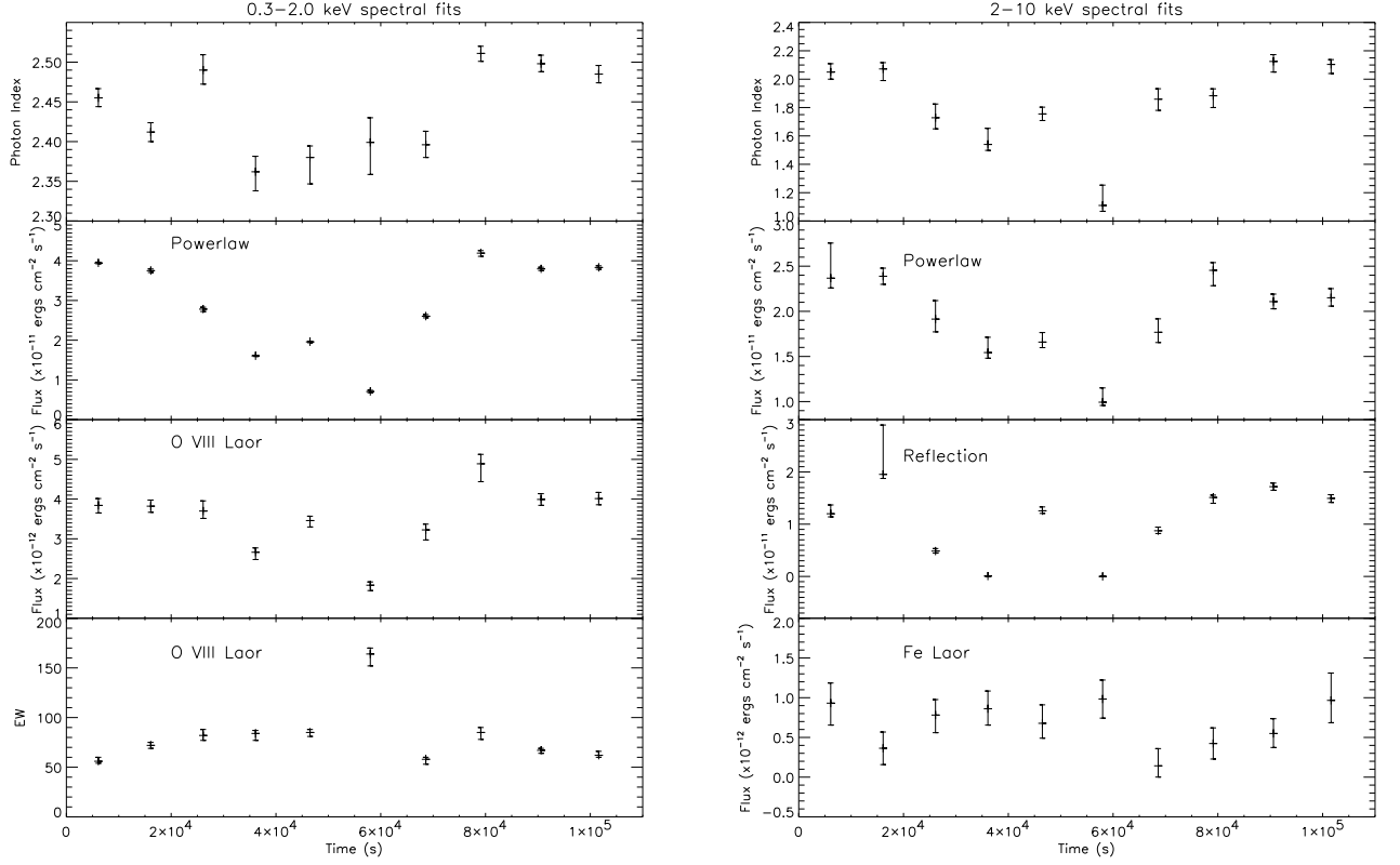
Figure 5.11: Left : Time resolved spectral analysis results for the 0.3–2.0 keV range. Related variations are observed between the soft PL flux, the photon index and the O VIII Laor line flux. Right : Time resolved spectral analysis results over the 2.0–10.0 keV range. Related variations are observed between the PL flux, the photon index and the reflection flux. The iron line flux is relatively unvarying.
