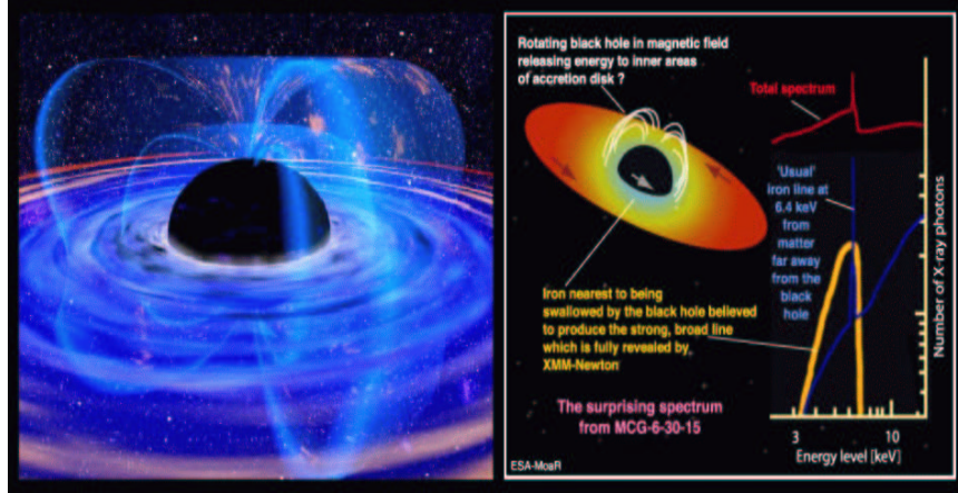
Figure 1.5: A schematic diagram of the innermost regions of the accretion disk (left) and on the right the X-ray spectrum showing the broad Fe K_\alpha line from the accretion disk around black holes ( credit : ESA image archive)
