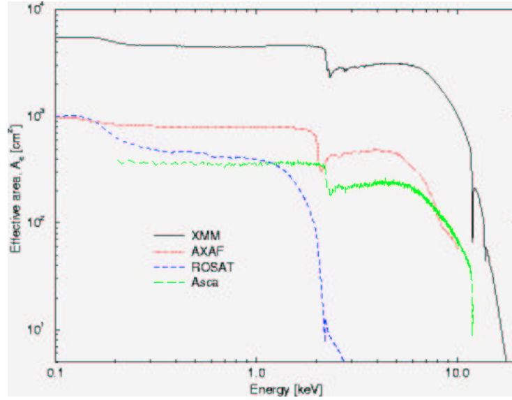
Figure 2.1: A comparison of the XMM-Newton mirror areas with those of of few recent X-ray observatories; credit : XMM-Newton users handbook & HEASARC
